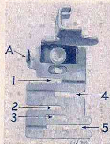
FIG. 48 THE EDGE-STITCHER
