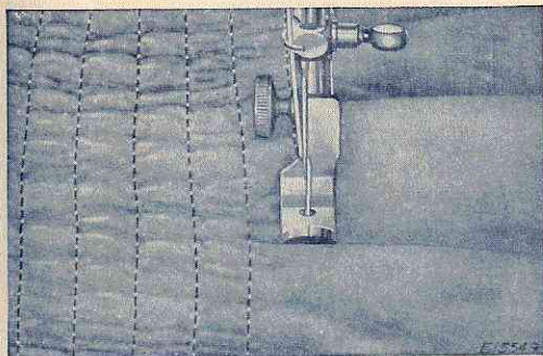
FIG. 56. THE GATHERER IN OPERATION
