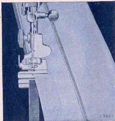
FIG. 51. PIPING WITH THE EDGE-STITCHER
