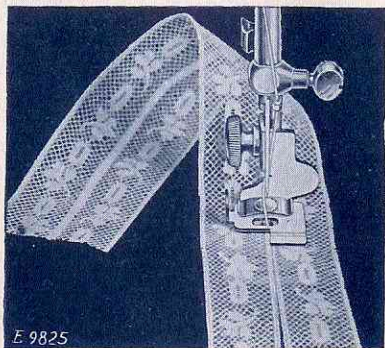
Fig. 49. SEWING LACE TOGETHER
