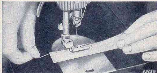
FIG. 36. MAKING A HEM WITH THE FOOT HEMMER
