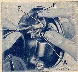
FIG. 6. ADJUSTMENT OF BOBBIN WINDER
