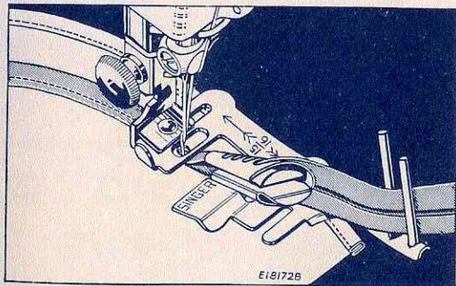
FIG. 47. APPLYING A FRENCH FOLD
