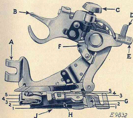
FIG. 59. THE RUFFLER AND ITS PARTS
