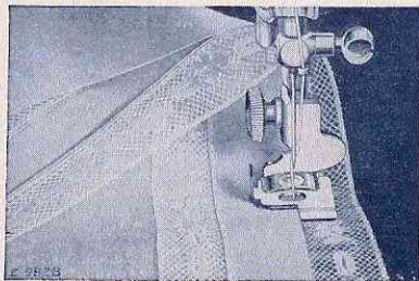
Fig. 50. SETTING IN LACE INSERTION
