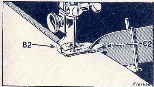
FIG. 43 BINDING WITH UNFOLDED BINDING
