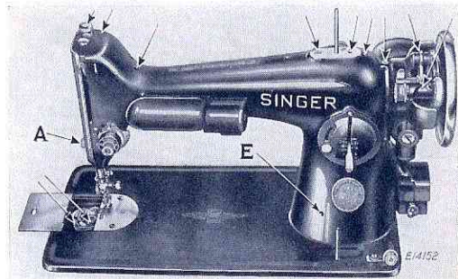
FIG. 23. FRONT VIEW, SHOWING OILING POINTS
