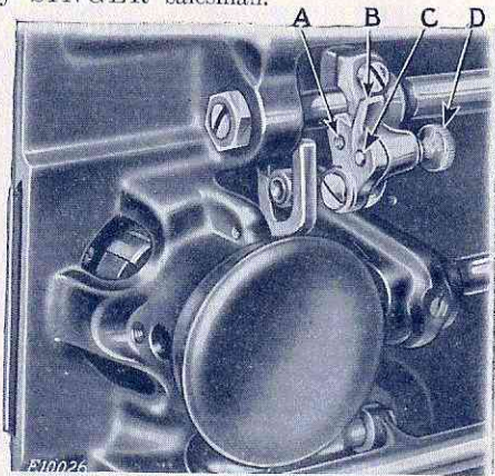
FIG. 31. ADJUSTMENT FOR DARNING OR EMBROIDERING
