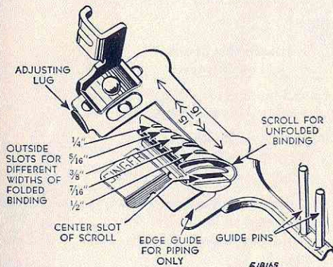
Fig. 41. MULTIPLE SLOTTED BINDER 160359
