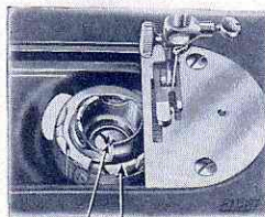
FIG. 24 VIEW OF SEWING HOOK SHOWING OILING POINTS
