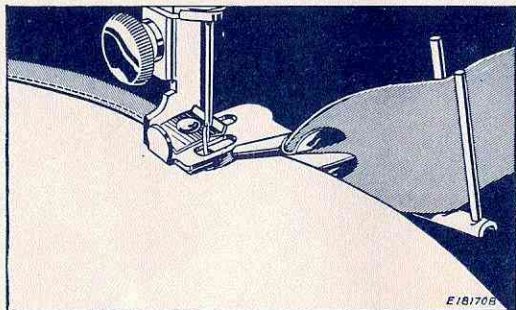
FIG. 46. BINDING AN OUTSIDE CURVE
