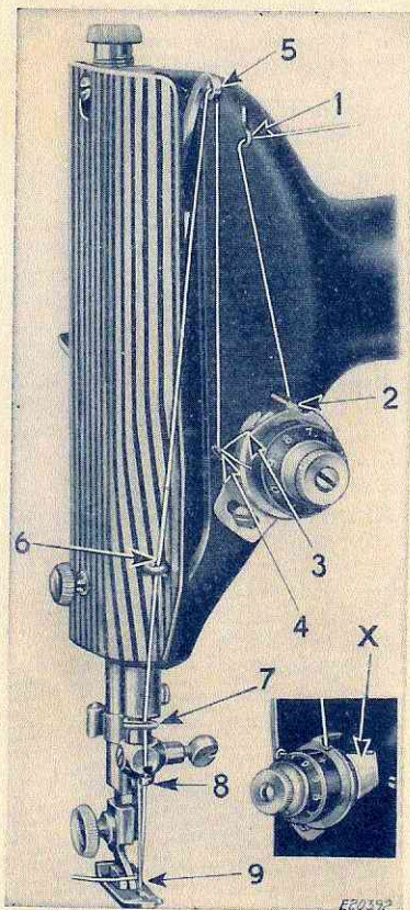
FIG. 12. UPPER THREADING
