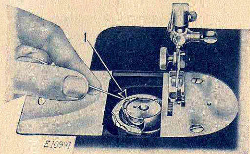
FIG. 8. THREADING THE BOBBIN CASE
