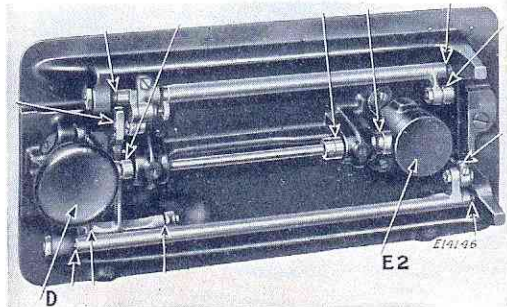
FIG. 28. OILING POINTS IN BASE OF MACHINE
