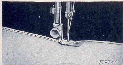
FIG. 37. MAKING A HEMMED SEAM
