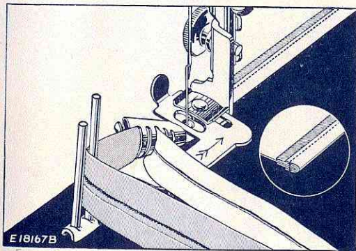
Fig. 45. PIPING AND BINDING IN ONE OPERATION
