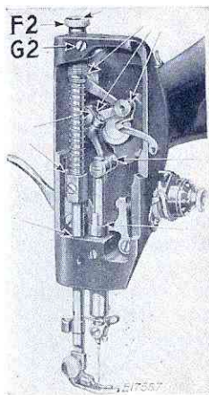
FIG. 27. END VIEW SHOWING OILING POINTS
